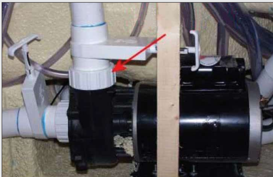
FIGURE 1.5 : PUMP UNION; LOOSEN UP TO BLEED AIR
